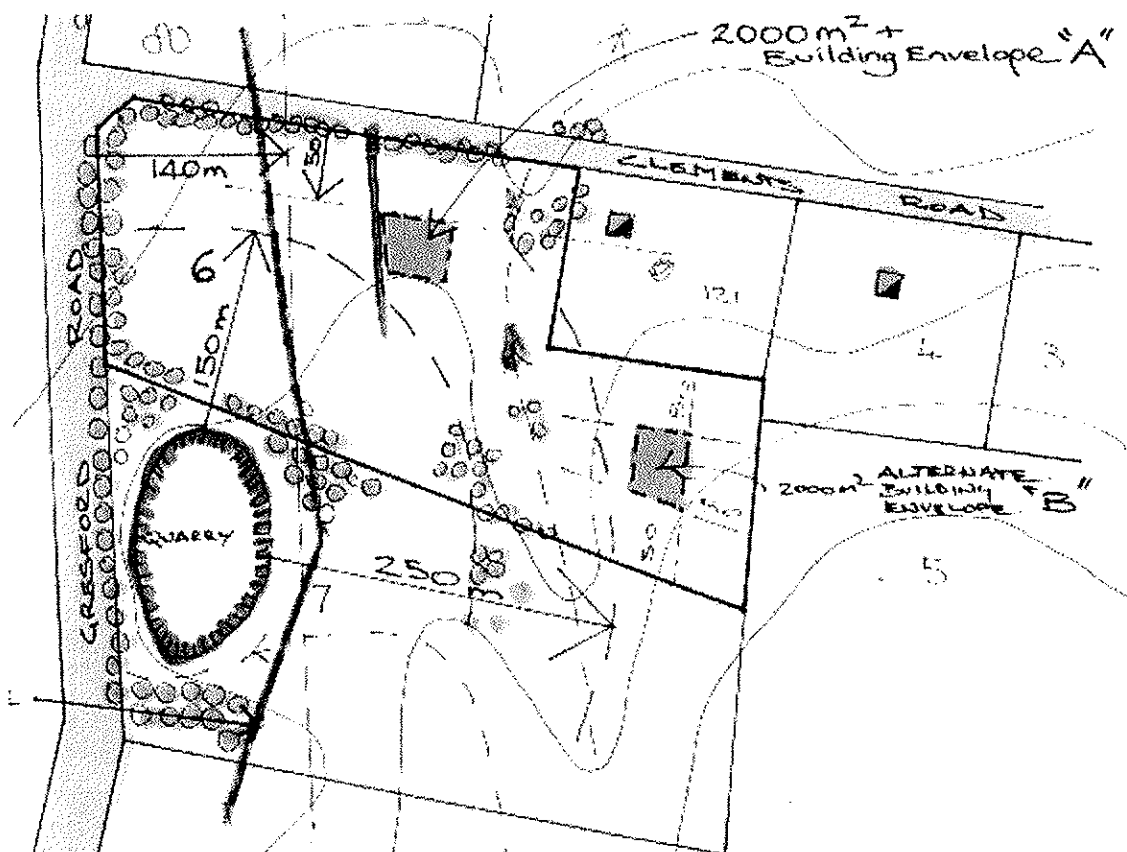
Figure 4: Lot 6 DP 248699 – Proposed Building Envelopes
